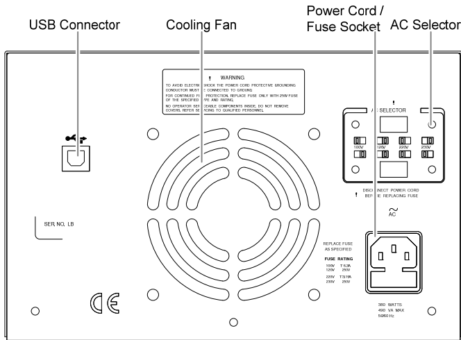
USB Connector
